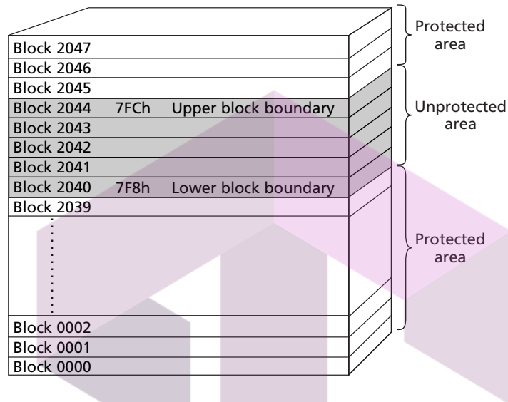
Figure 56: Flash Array Protected: Invert Area Bit = 1
